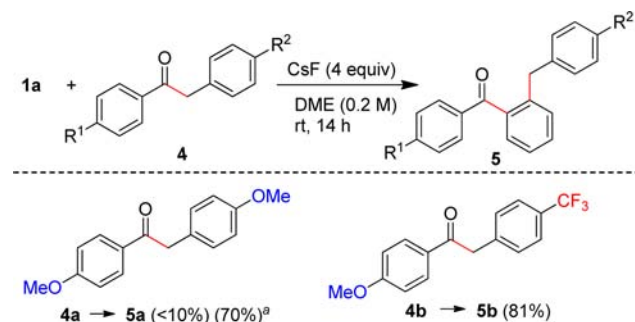
Scheme 2. Investigation of the Electronic Influence of Benzylic Ketones on the Conversion
