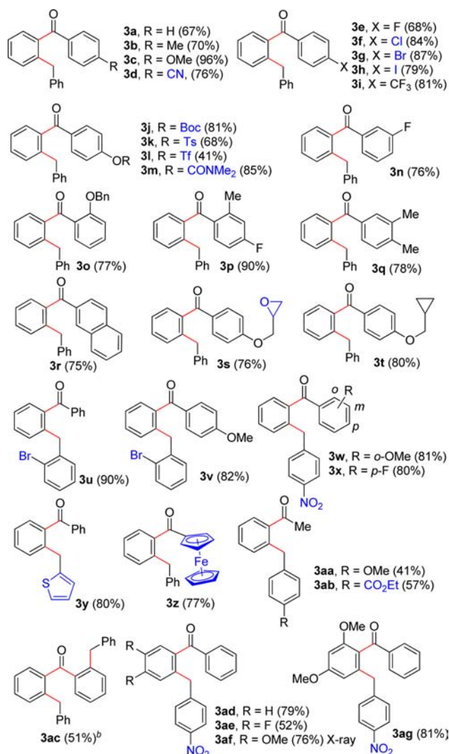
Figure 1. Aryne insertion into C–C bonds for the synthesis of 2-benzylphenyl ketones. (a) Conditions: aryne precursor (0.4 mmol), ketone (0.2 mmol), CsF (0.8 mmol), DME (1 mL), rt, 6–16 h. Isolated yield was given. (b) 1a (0.8 mmol), 24 h.
