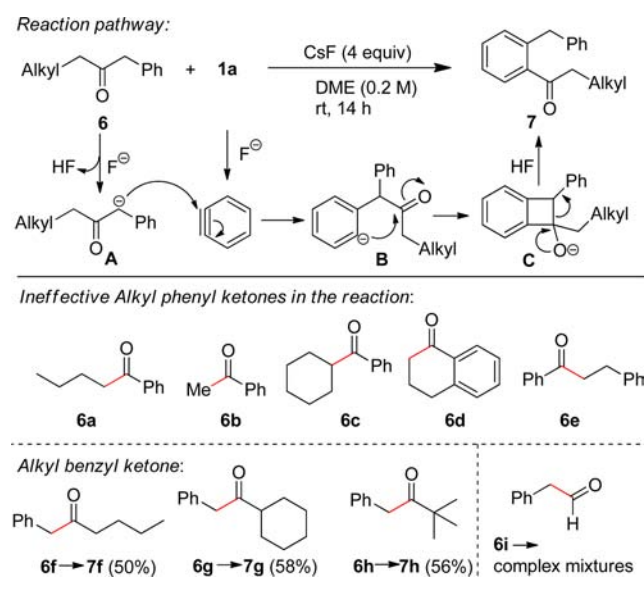
Scheme 3. Mechanistic Insights
